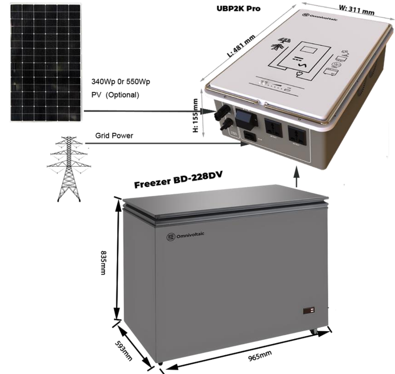
UBP1K pro and UBP2K pro and 228L Freezer Pack
