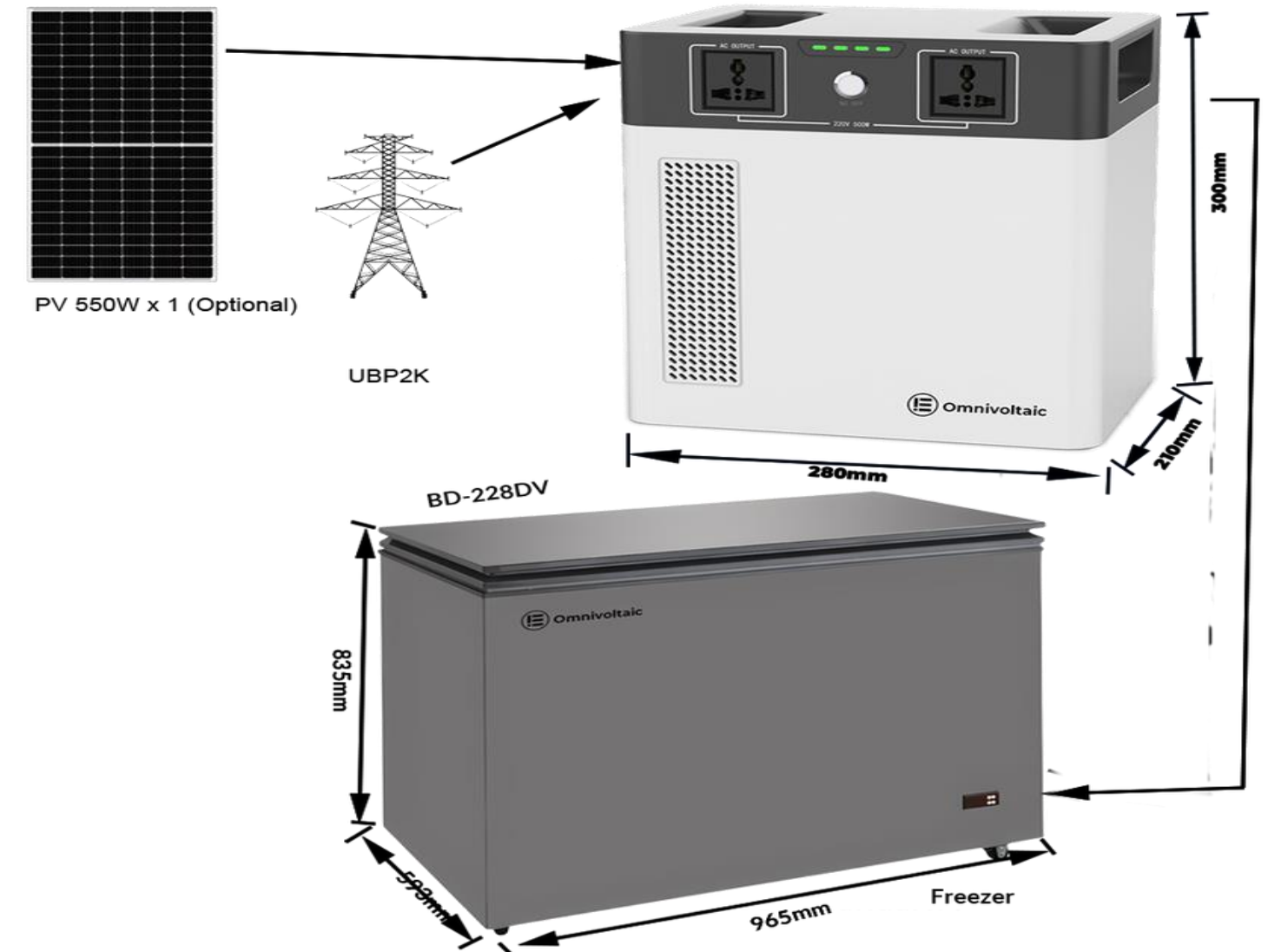
UBP1K and UBP2K and 228L Freezer Pack
